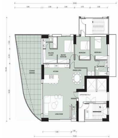
1st FLOOR PLAN SCALE 1:100
