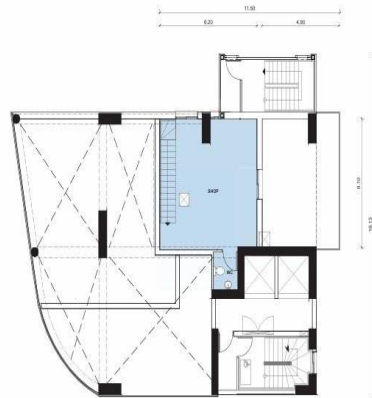
MIDDLE FLOOR PLAN SCALE 1:100
