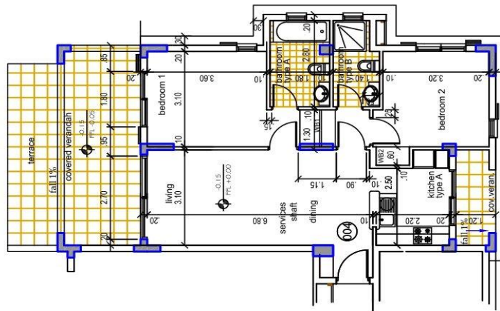
APARTMENT PLAN
