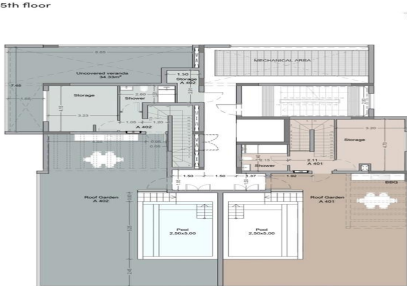
5th floor
