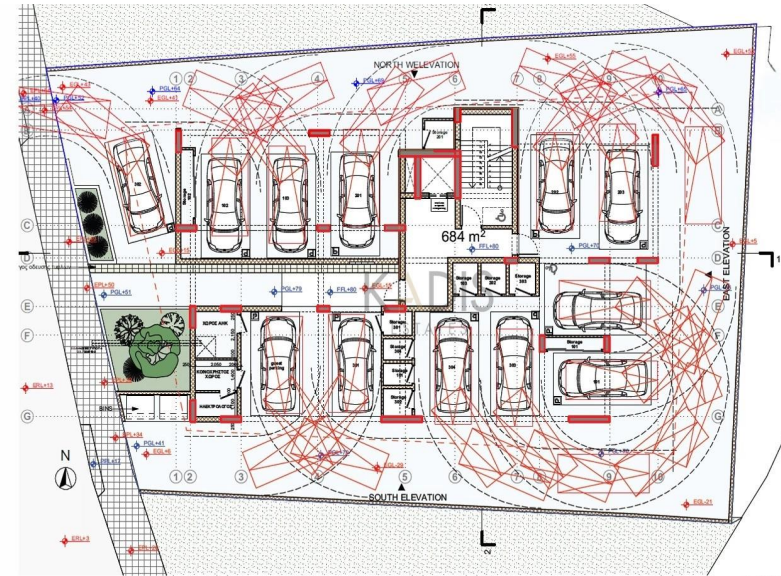
GROUND FLOOR PLAN 1:200
