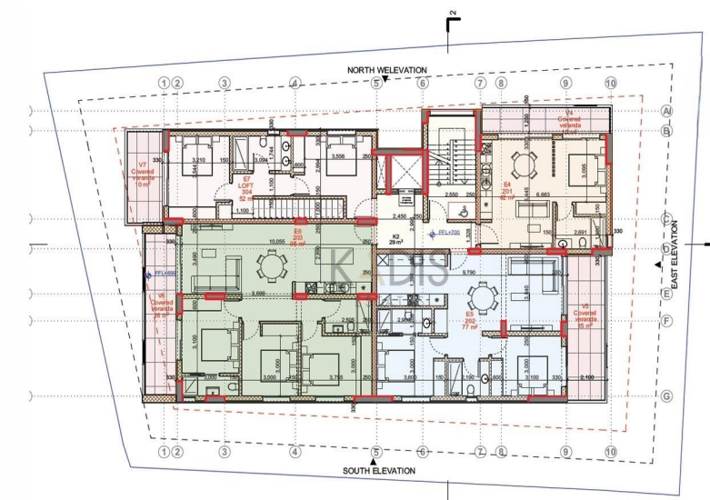
SECOND FLOOR PLAN 1:200
