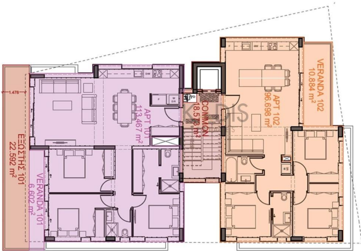
1 ST FLOOR
