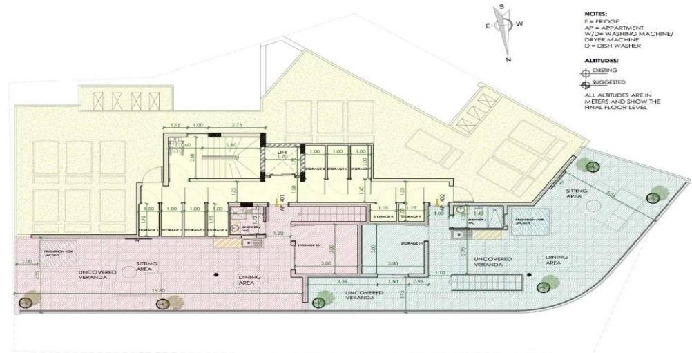
ARDEN ROOF FLOOR PLAN
