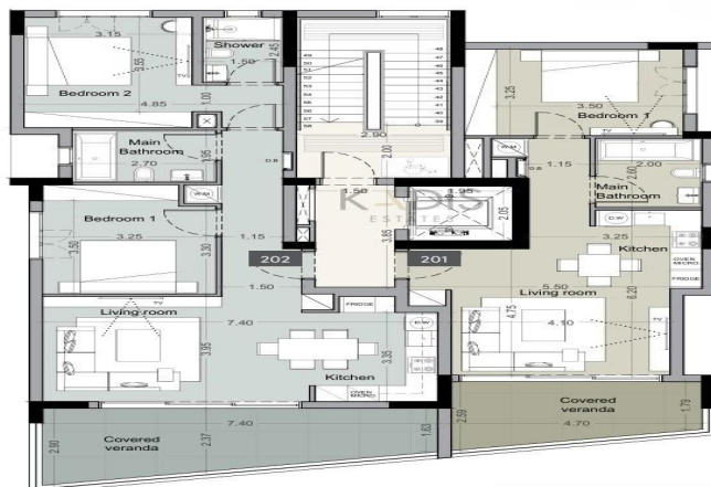
2nd floor
