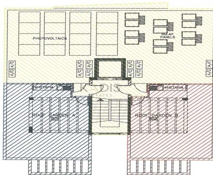
ROOF PLAN
