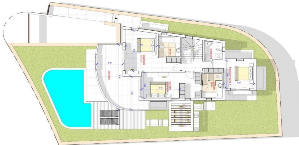
PRELIMINARY FIRST FLOOR
