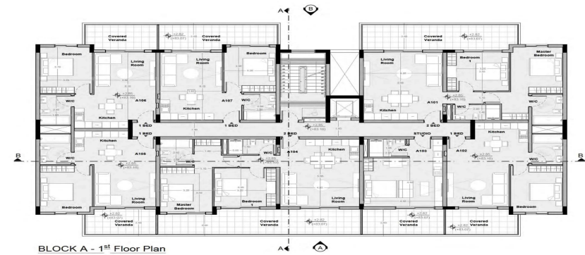
BLOCK A - 1st Floor Plan
