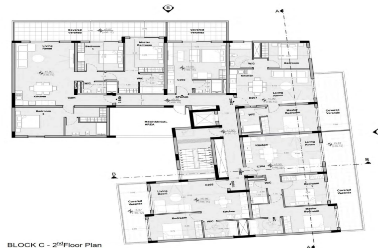
BLOCK C - 2 nd Floor Plan
