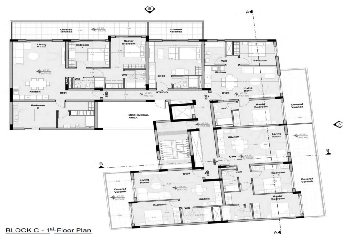
BLOCK C - 1 st Floor Plan
