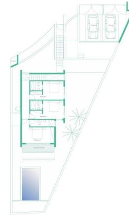
First Floor 85 s.m.
