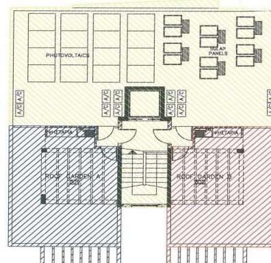
ROOF PLAN
