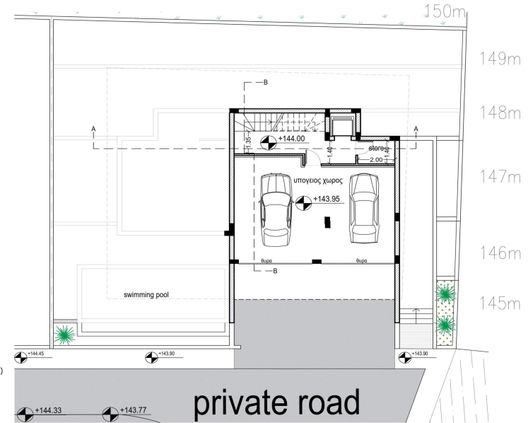
basement Es 25.28m 2 (-1.96m 2 ) Euvr = 56.53m 2 Ecov.ver. = 30.50m 2
