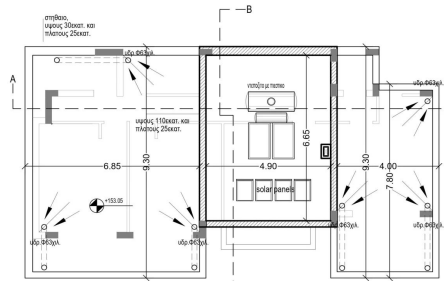
roof plan
