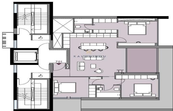
3 Bedroom Apartment | 701
