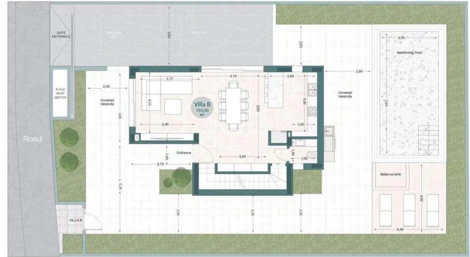
VILLA B GROUND FLOOR
