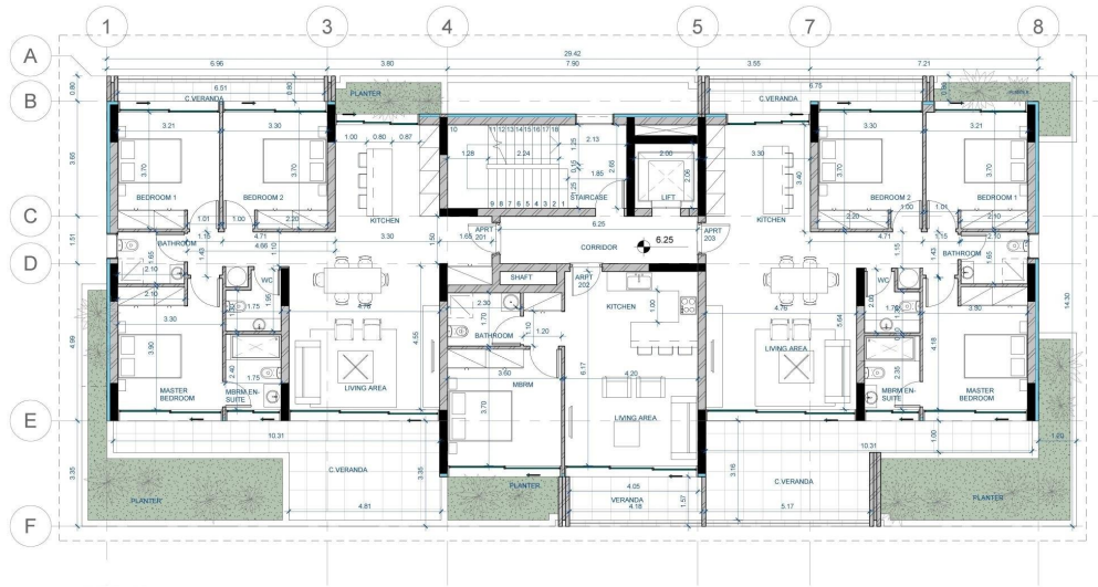
BLOCK B & D SECOND FLOOR SCALE 1 100
