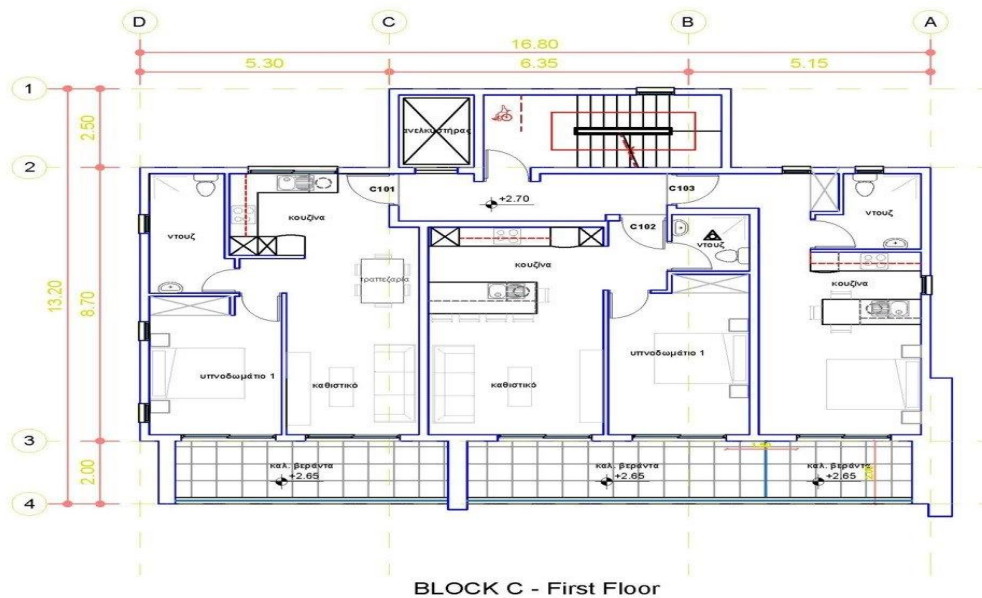
BLOCK C - First Floor
