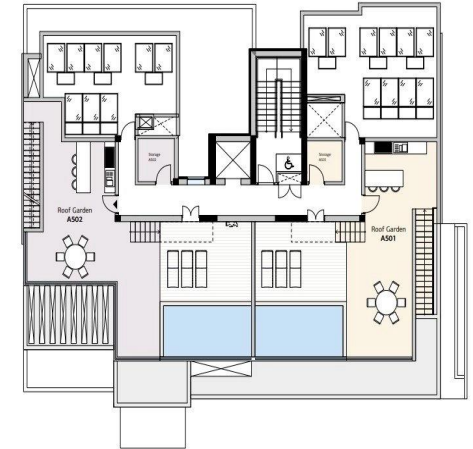
BLOCK A - B ROOF GARDEN
