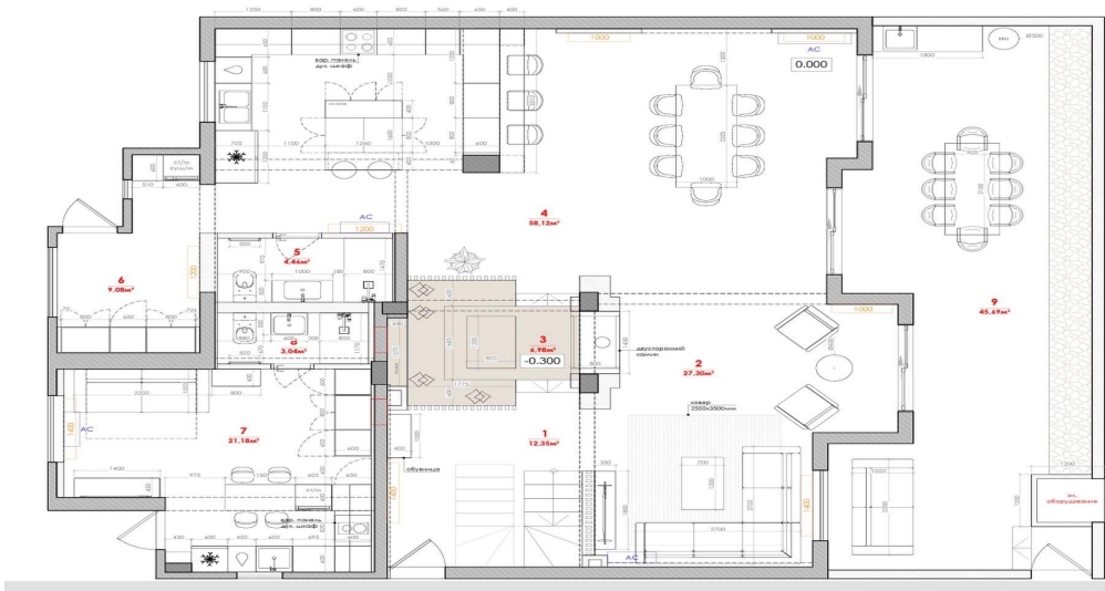
GROUND FLOOR DESIGN PROJECT
