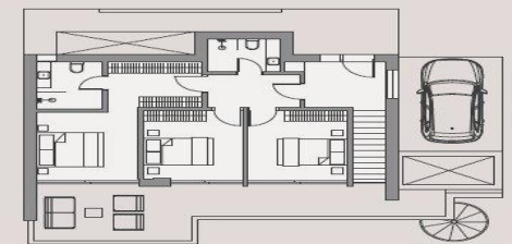
FIRST FLOOR
