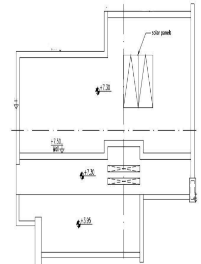
ROOF PLAN
