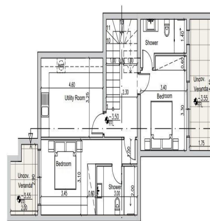
BASEMENT FLOOR
