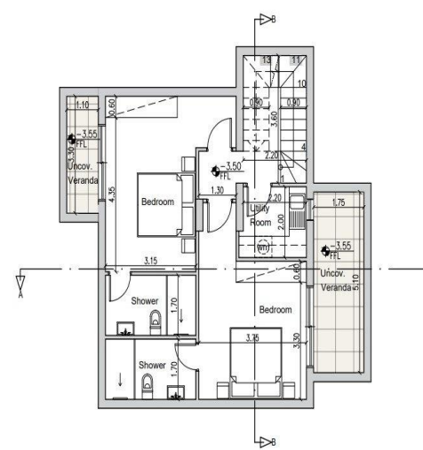
BASEMENT FLOOR
