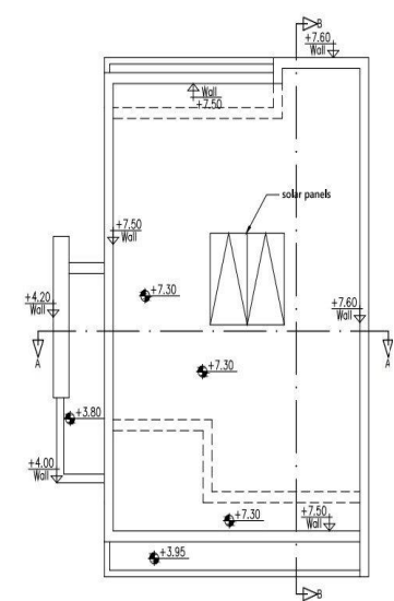
ROOF PLAN
