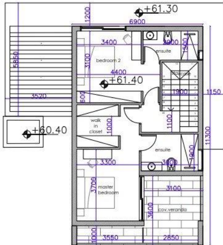
FIRST FLOOR SCALE 1:100
