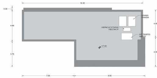
ROOF PLAN
