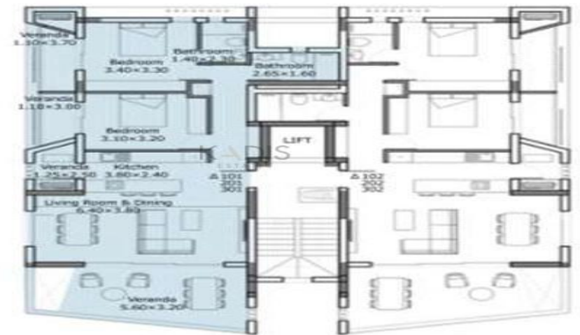
TYPICAL FLOORS PLAN
