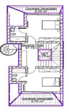
SECOND FLOOR BUILT AREA = 67.76sq m
