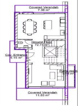
GROUND FLOOR BUILT AREA = 72.74sq m
