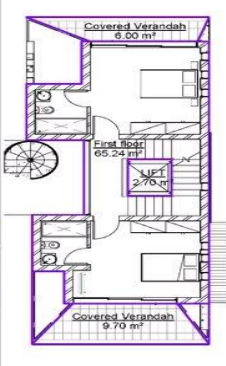
FIRST FLOOR BUILT AREA = 65.24sq m
