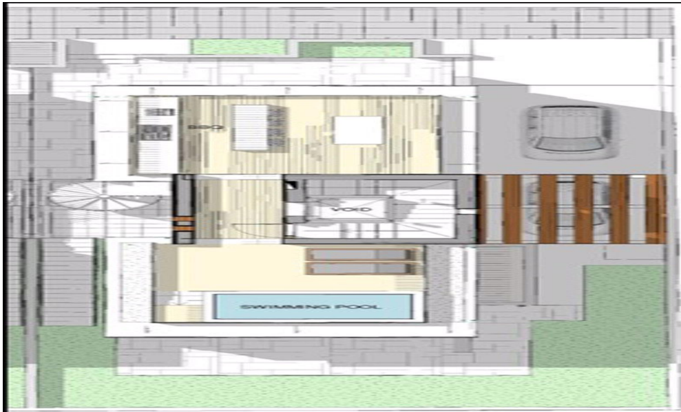
GROUND FLOOR BUILT AREA = 72.74sq m
