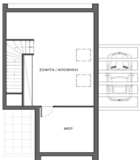
ATTIC PLAN
