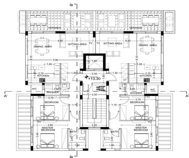
FOURTH FLOOR
