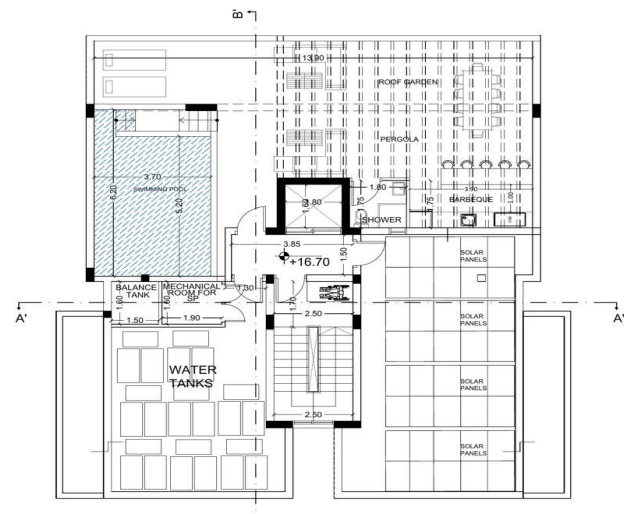
ROOF PLAN
