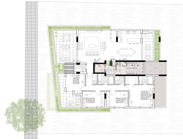
5 th Floor
