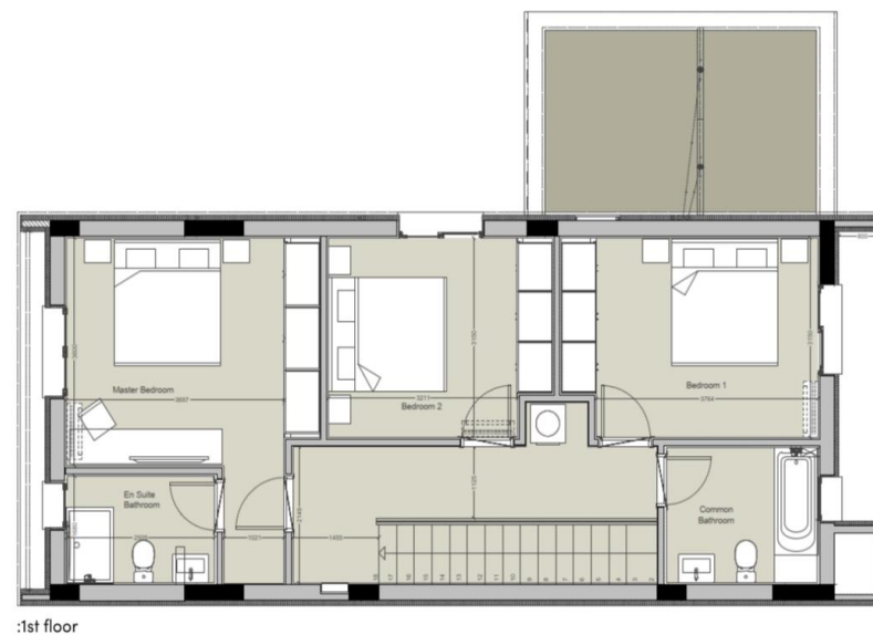
floor plans H2
