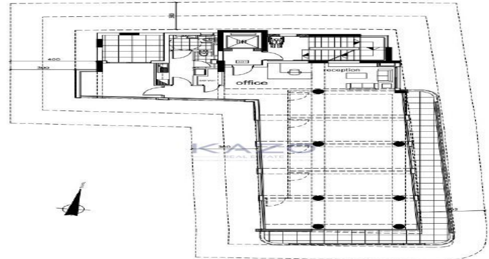
3rd floor plan BUILDING COEFFICIENT = 196.29 M 2 COVERED VERANDAS ....= 45.32 M 2
