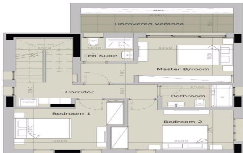
1st floor
