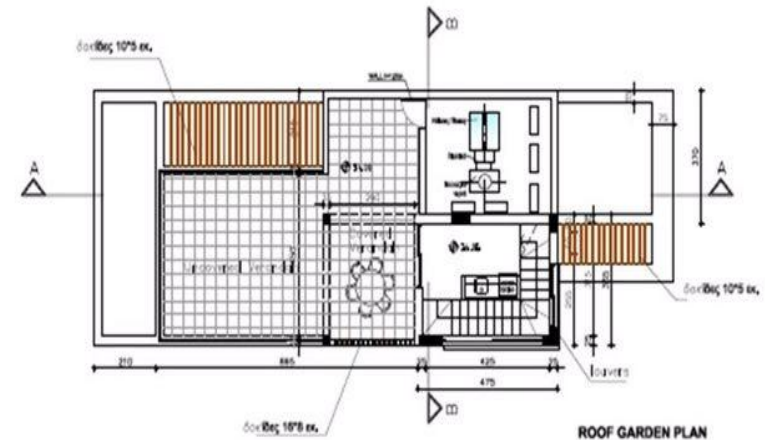
ROOF GARDEN PLAN
