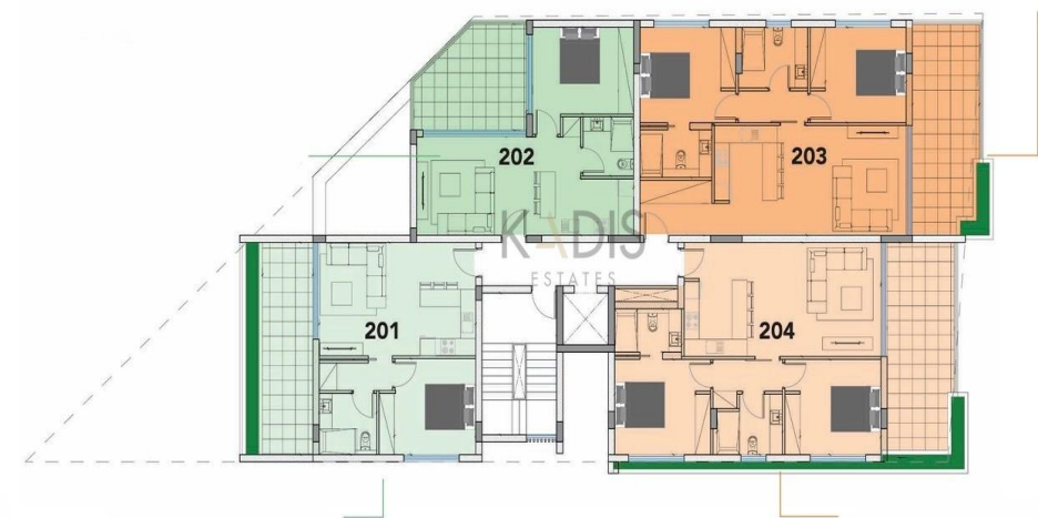
SECOND FLOOR
