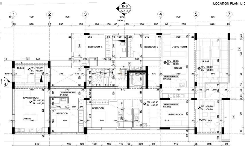
LOCATION PLAN 1:10
