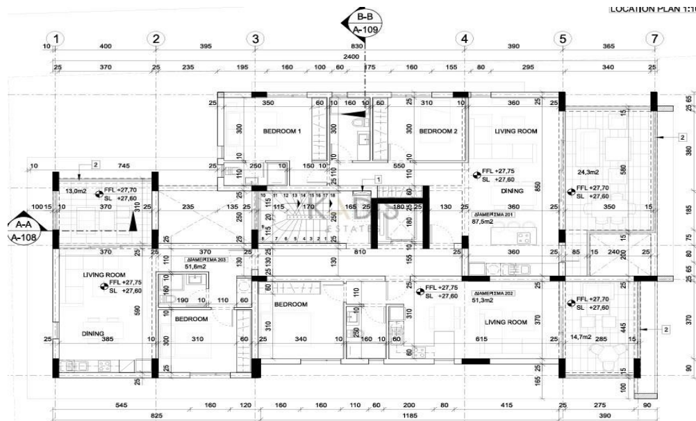
LOCATION PLAN 1:10
