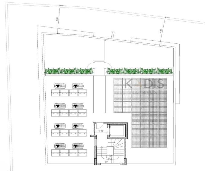
FLOOR PLANS [Roof]
