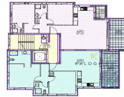
1 Second Floor 1:100
