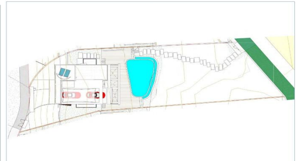
PRELIMINARY SITE PLAN
