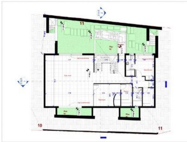
PRELIMINARY LOWER GROUND FLOOR PLAN
