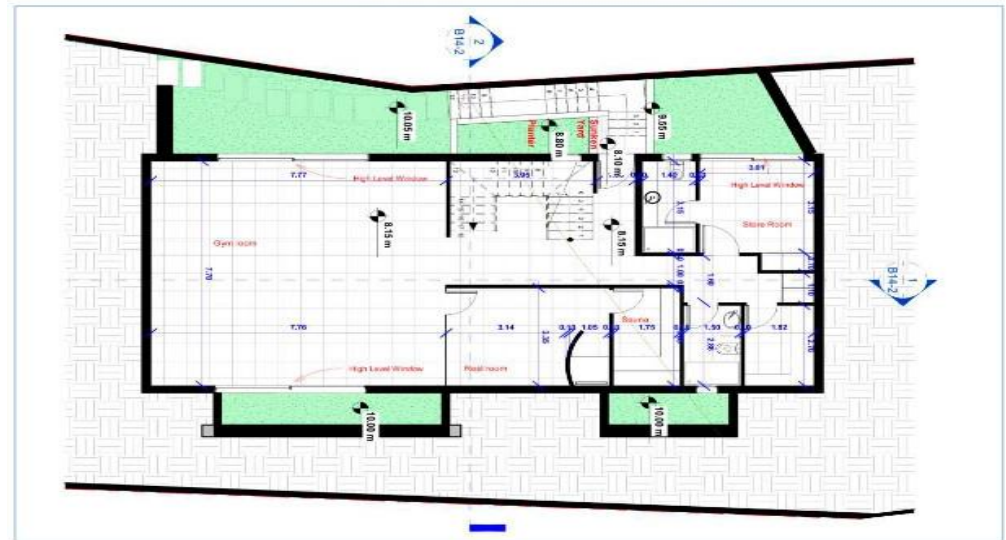
PRELIMINARY LOWER GROUND FLOOR PLAN
