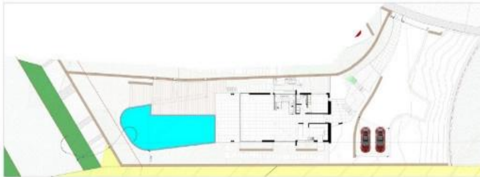
PRELIMINARY GROUND FLOOR PLAN
