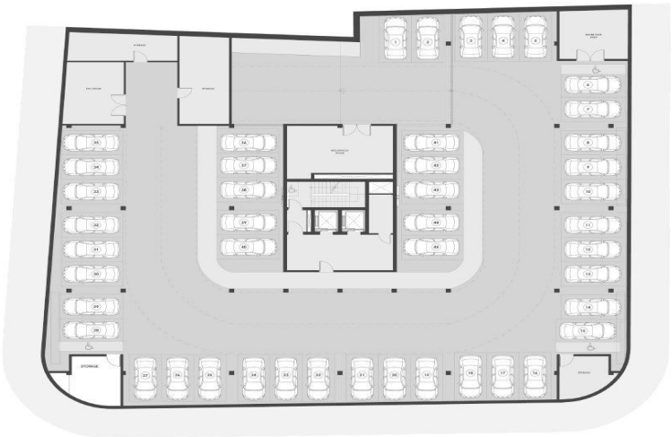
BASEMENT
