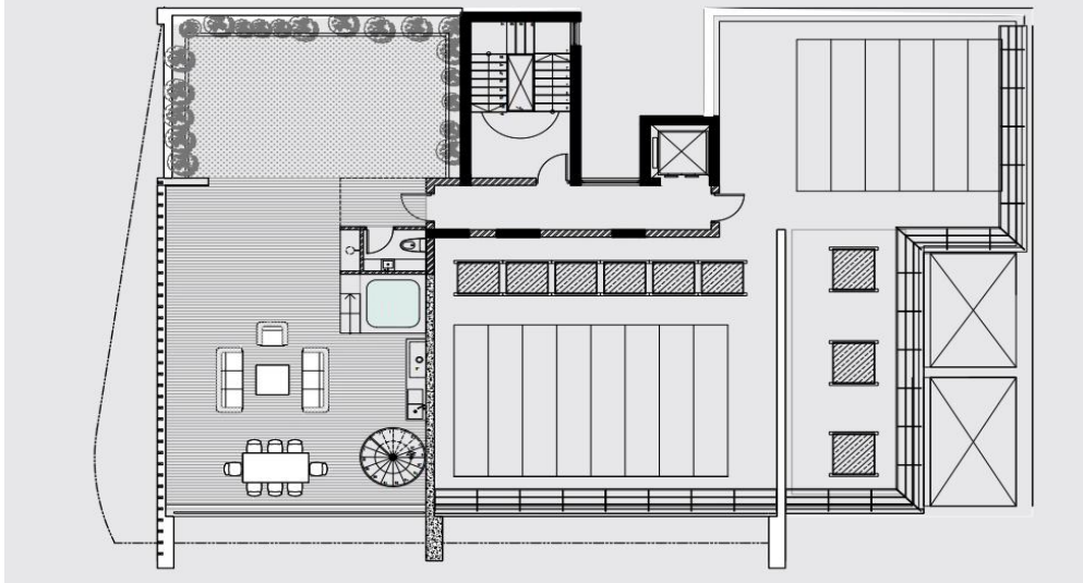
Typical Roof Plan
