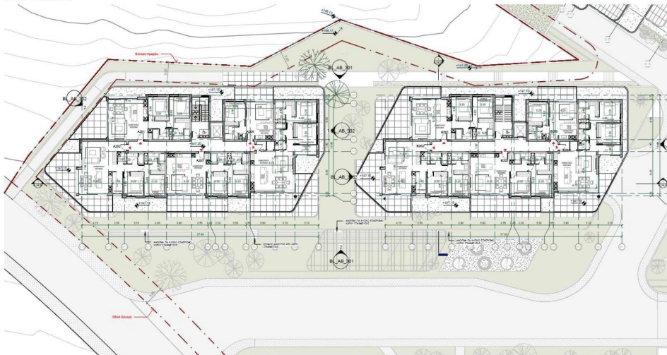
2ND FLOOR
