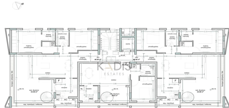
3RD FLOOR
