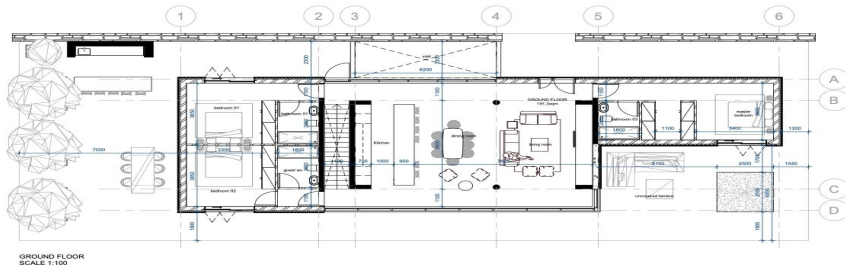
GROUND FLOOR SCALE 1:100
