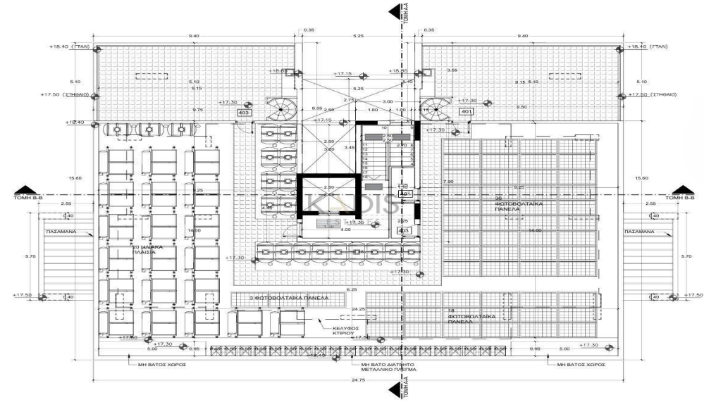
ROOF PLAN
