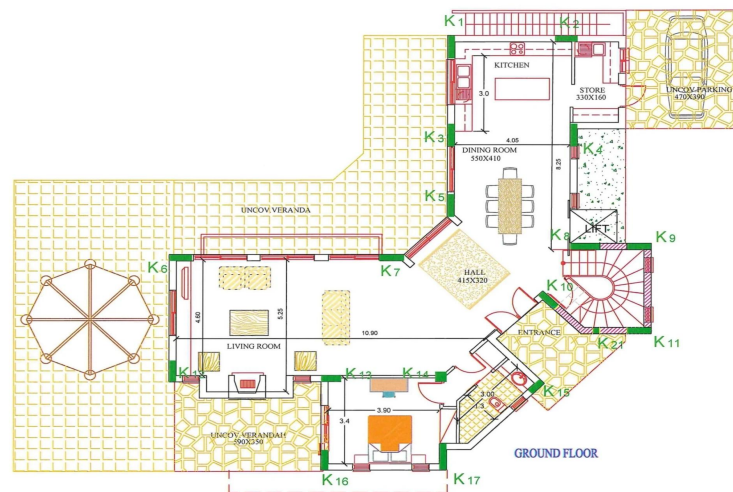
GROUND FLOOR 2nd OPTION (extra bedroom)
