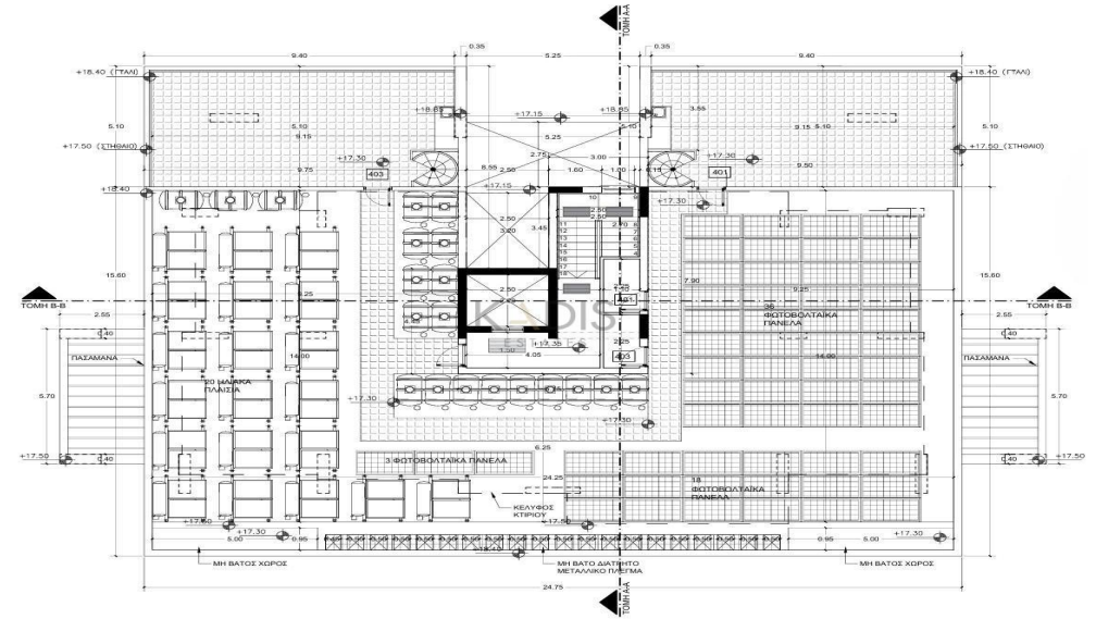
ROOF PLAN
